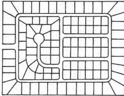
Image 1: Conventional subdivision design.
